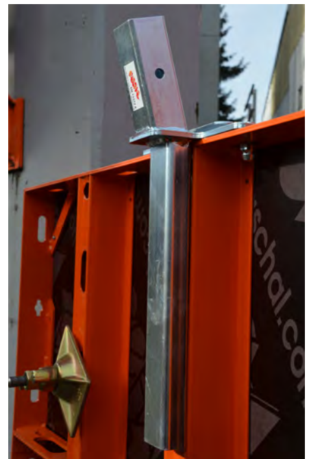
PASCHAL Secuset is easily assembled with the matching support when used with the lightweight formwork NeoR. Therefore the keybolt again serves as a light and friction-locked connection piece.
